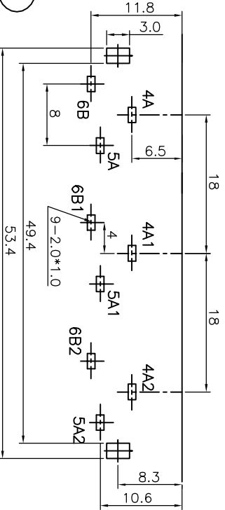
P.C.B.LAYOUT BOTTOM VIEW
